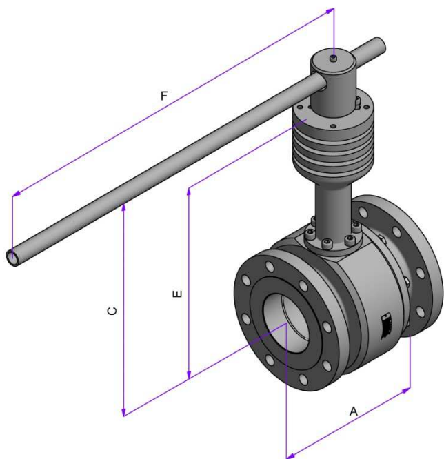
RF-RTJ
