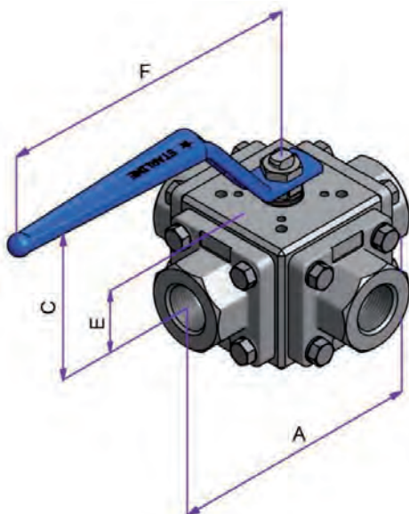
NPT-BSPP-BSPT
