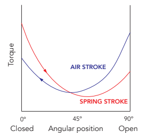
Symmetric yoke mechanism Spring to open
