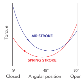
Symmetric yoke mechanism Spring to close
