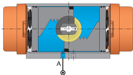
Central air chamber volume Double-Acting and Spring-Return
