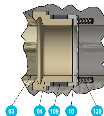
DETAIL SEAT
