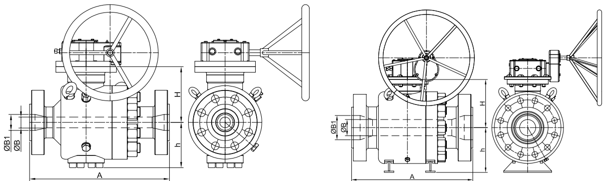
CLASS API 3000
