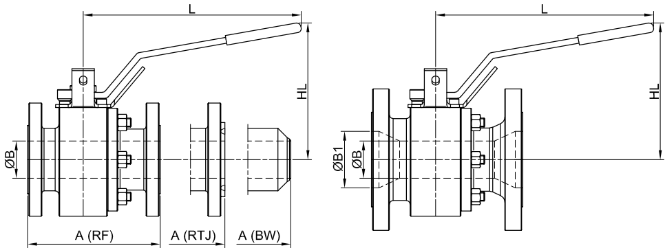
ASME CLASS 600
