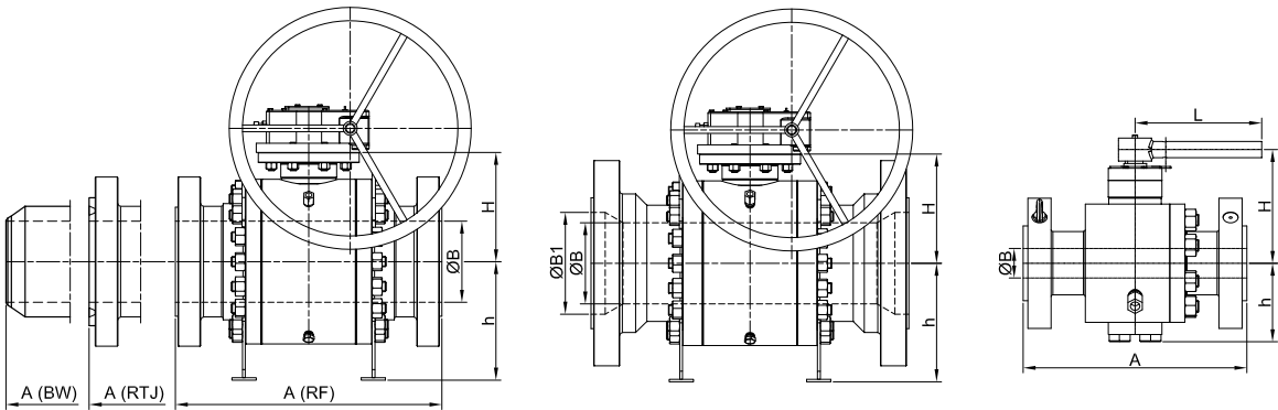
ASME CLASS 2500
