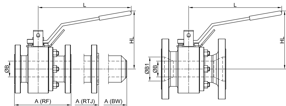
ASME CLASS 1500
