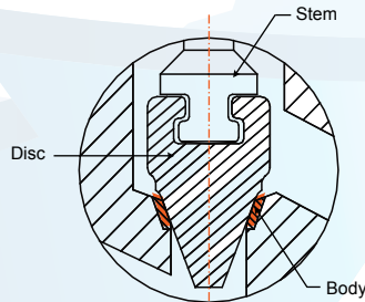
Needle Point Metering Plug
